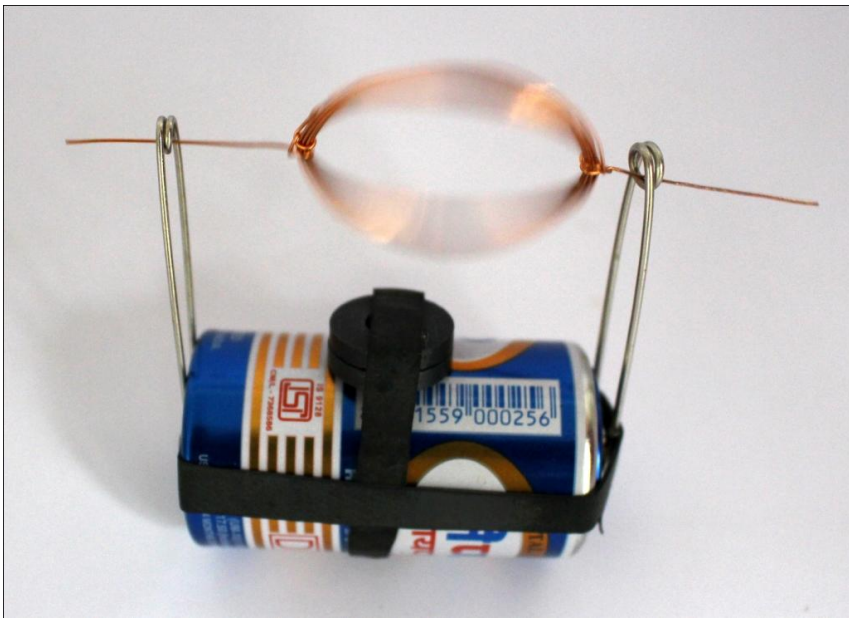
Figure 1. A glowing copper ring suspended by thin wires above a battery.
